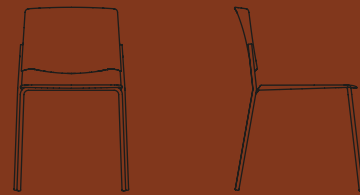
4 LEGS OPEN BACK CHAIR W 505 H 805 D 565
