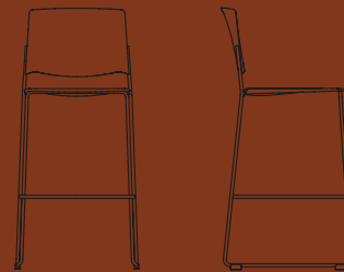
SLEDGE OPEN BACK SEAT W 520/525 H 1005/1105 D 540/552
